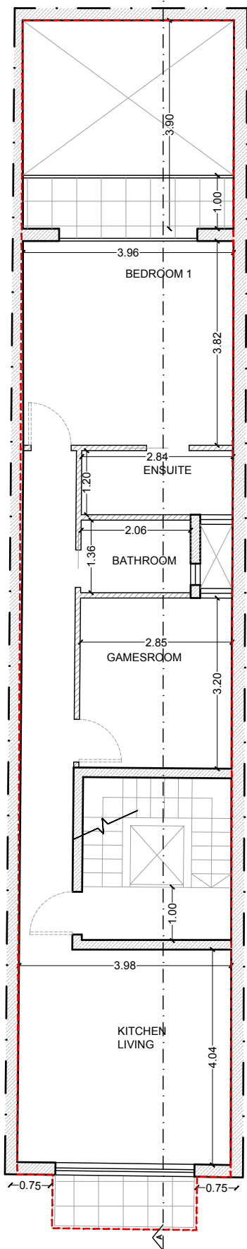
Proposed third floor plan
